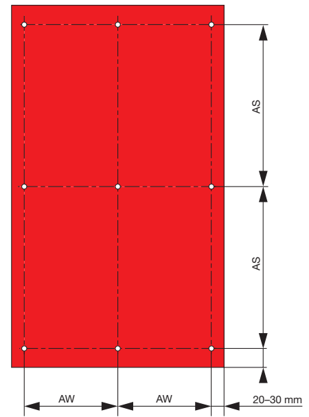
FASTENING DISTANCES
